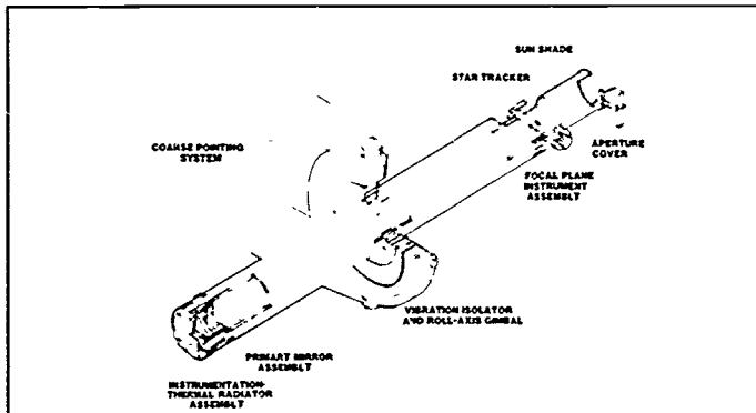
Astrometric Telescope Facility, which would search for planetary systems around other stars, could operate as an attached payload on Freedom's upper keel.
