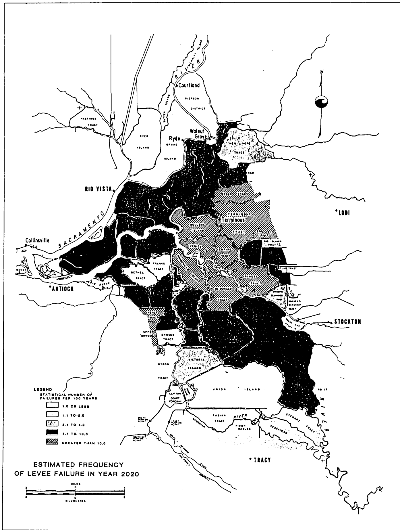
FIGURE 9 ESTIMATED LEVEE FAILURE FREQUENCIES IN 2020
