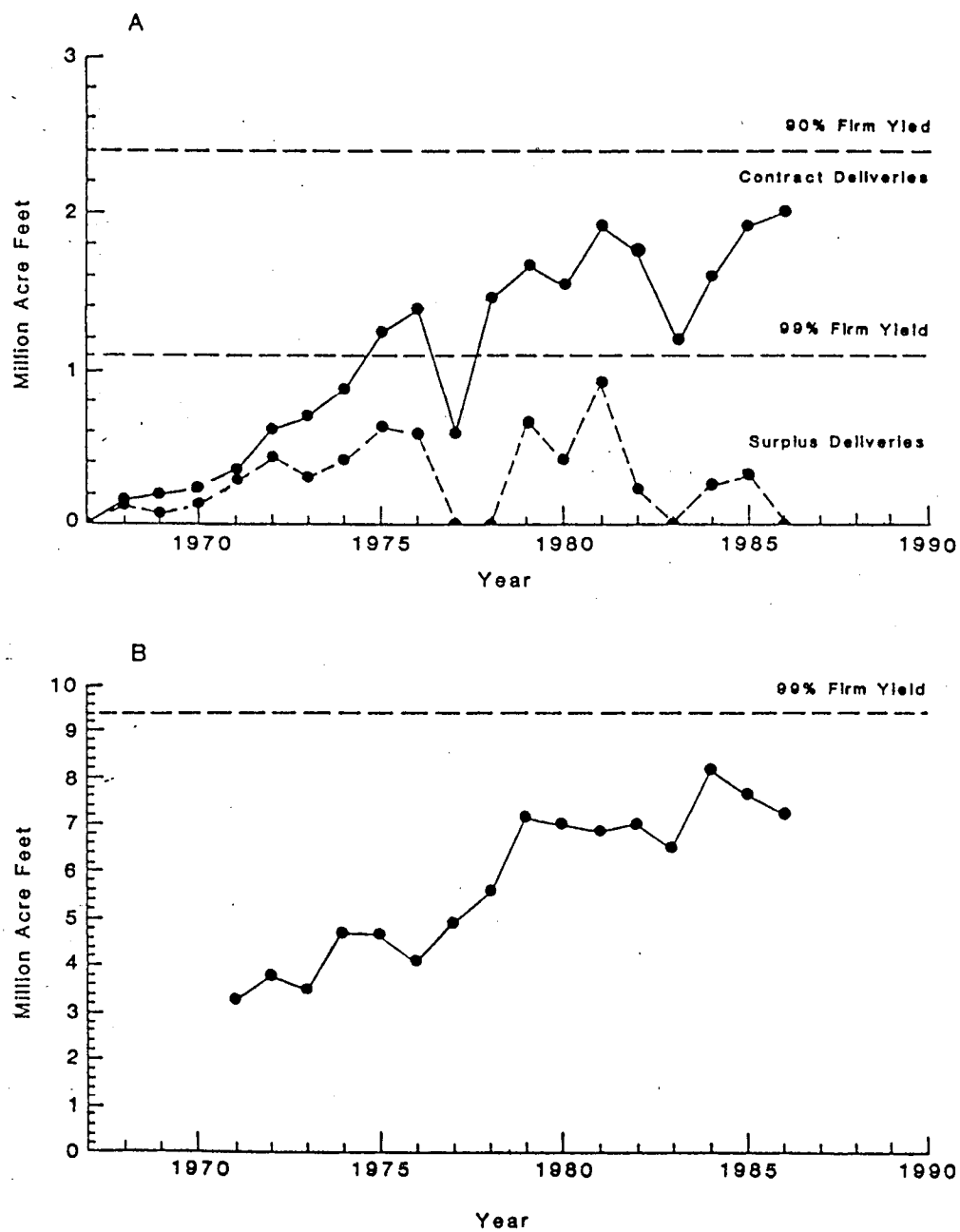
Figure 2. Water deliveries and firm yield levels for (a) the State Water Project and (b) the Central Valley Project.
