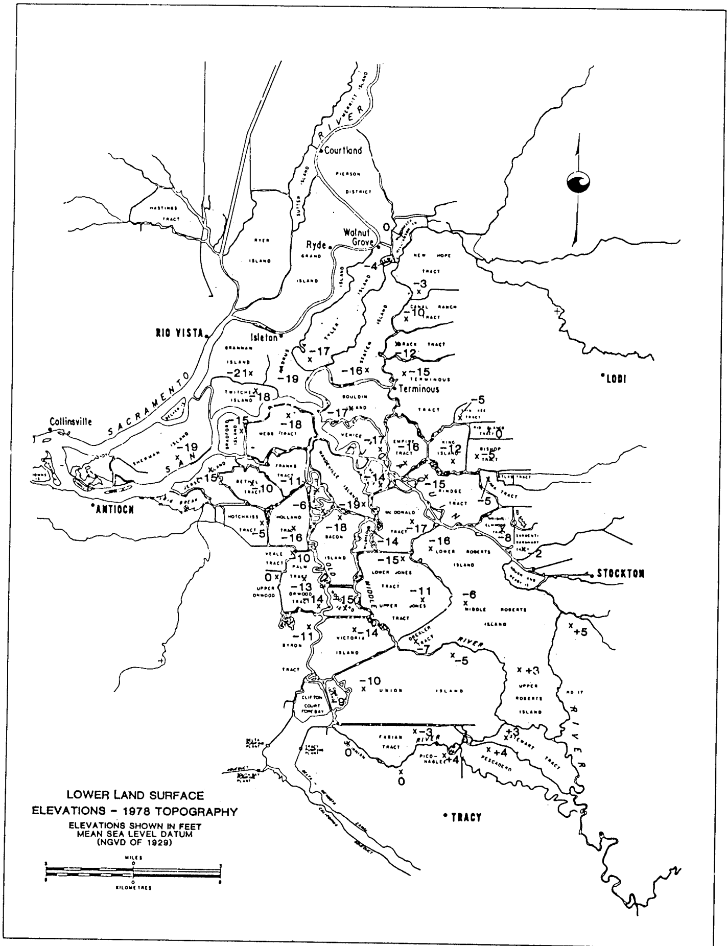
FIGURE 5 DELTA LAND ELEVATIONS SHOWING LANDS BELOW SEA LEVEL (minus values)
